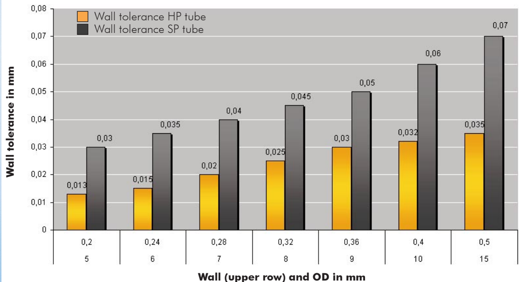
HP (High Precision) vs. SP (Standard Precision) Tube Tolerances
